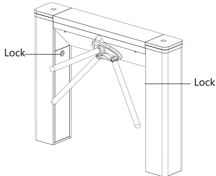
Figure 3-1 Lock Holes
