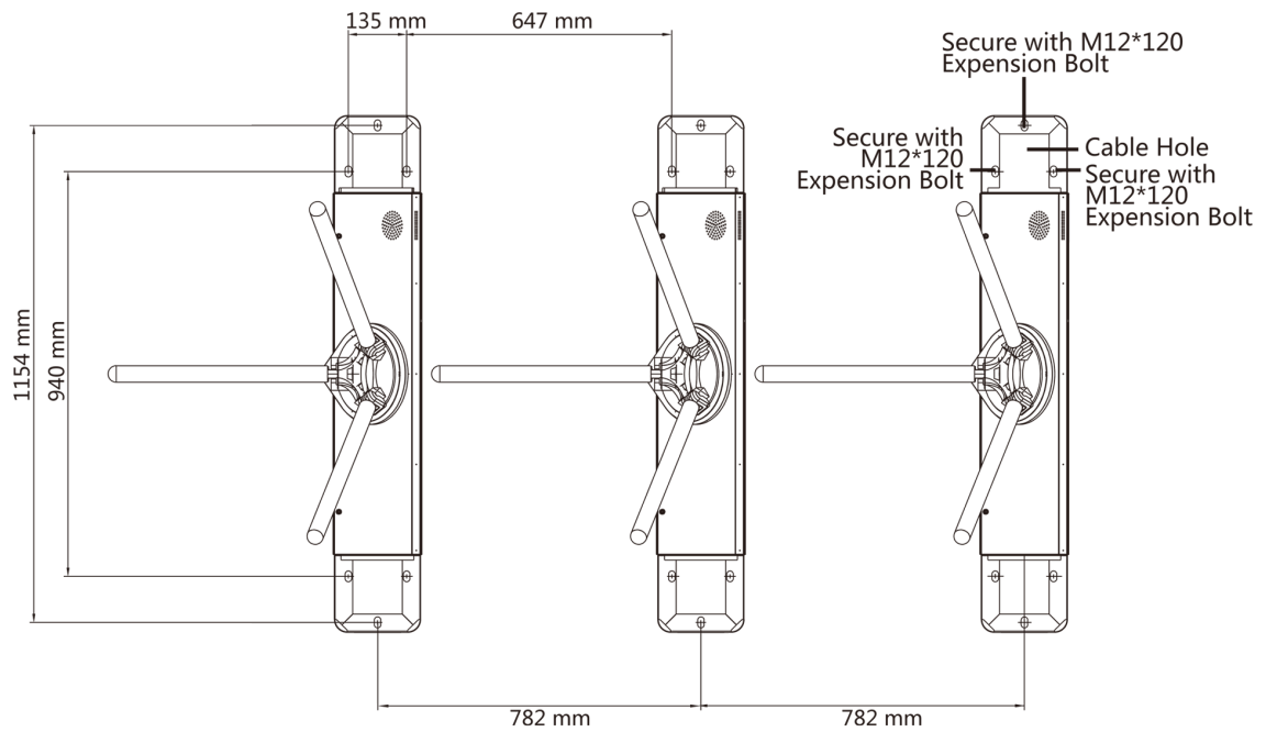
Figure 3-3 Installation Footprint
